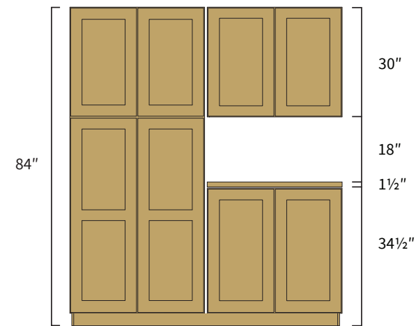
7' Ceiling
