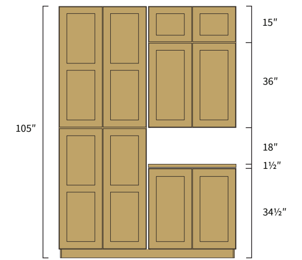
9' Ceiling
