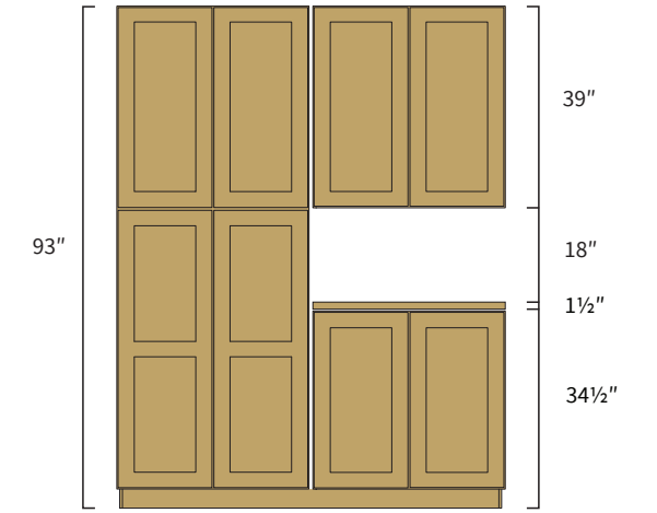
8' Ceiling With 39" Wall Cabinet
