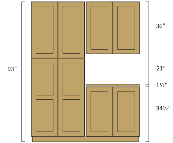
8' Ceiling With 36" Wall Cabinet
